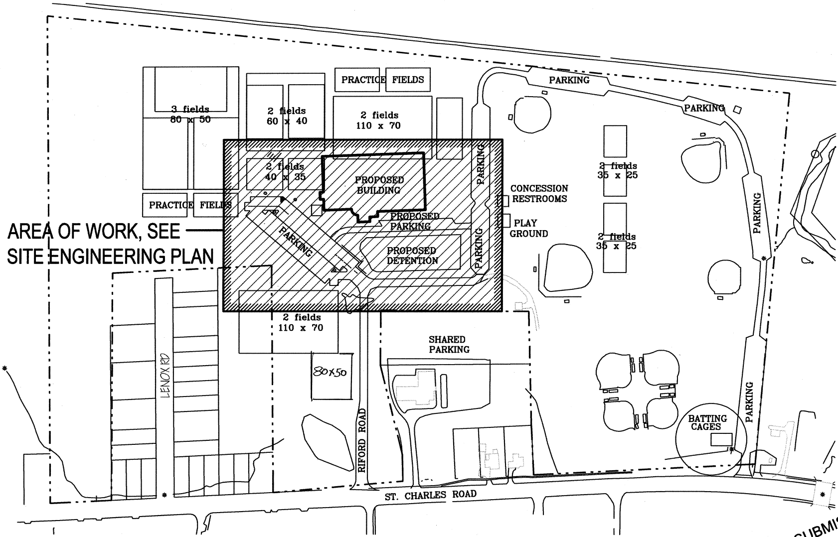
D6 OVERALL SCHEMATIC SITE PLAN SCALE: 1" = 200'-0"
